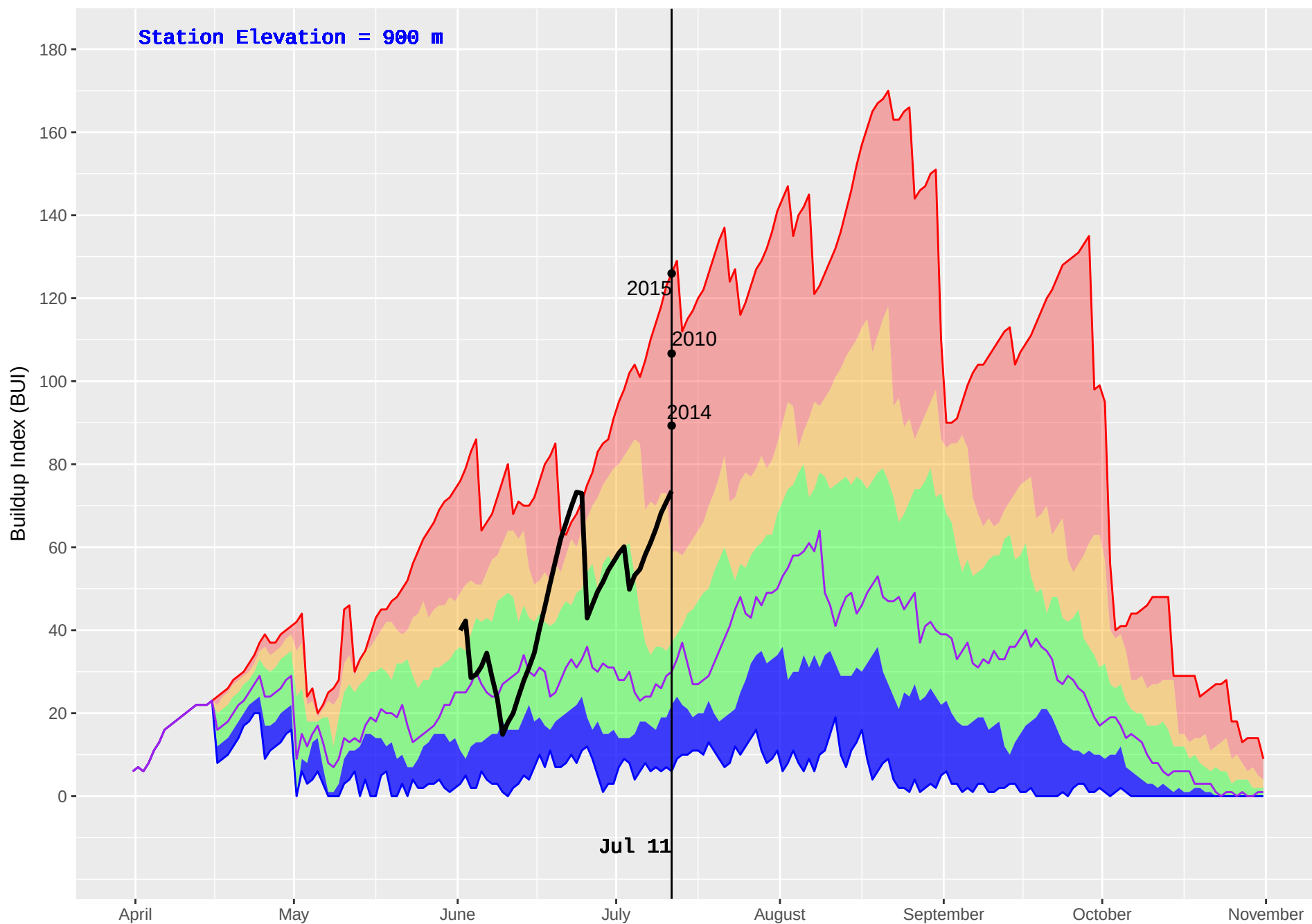
UPPER FULTON (169) : Historical (1986–2016) and Current (2018) Noon Buildup Index (BUI)
