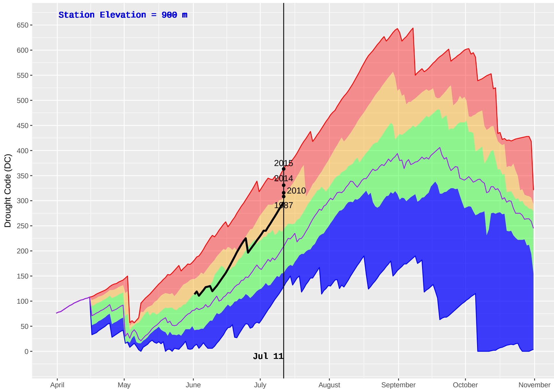
UPPER FULTON (169) : Historical (1986–2016) and Current (2018) Noon Drought Code (DC)
