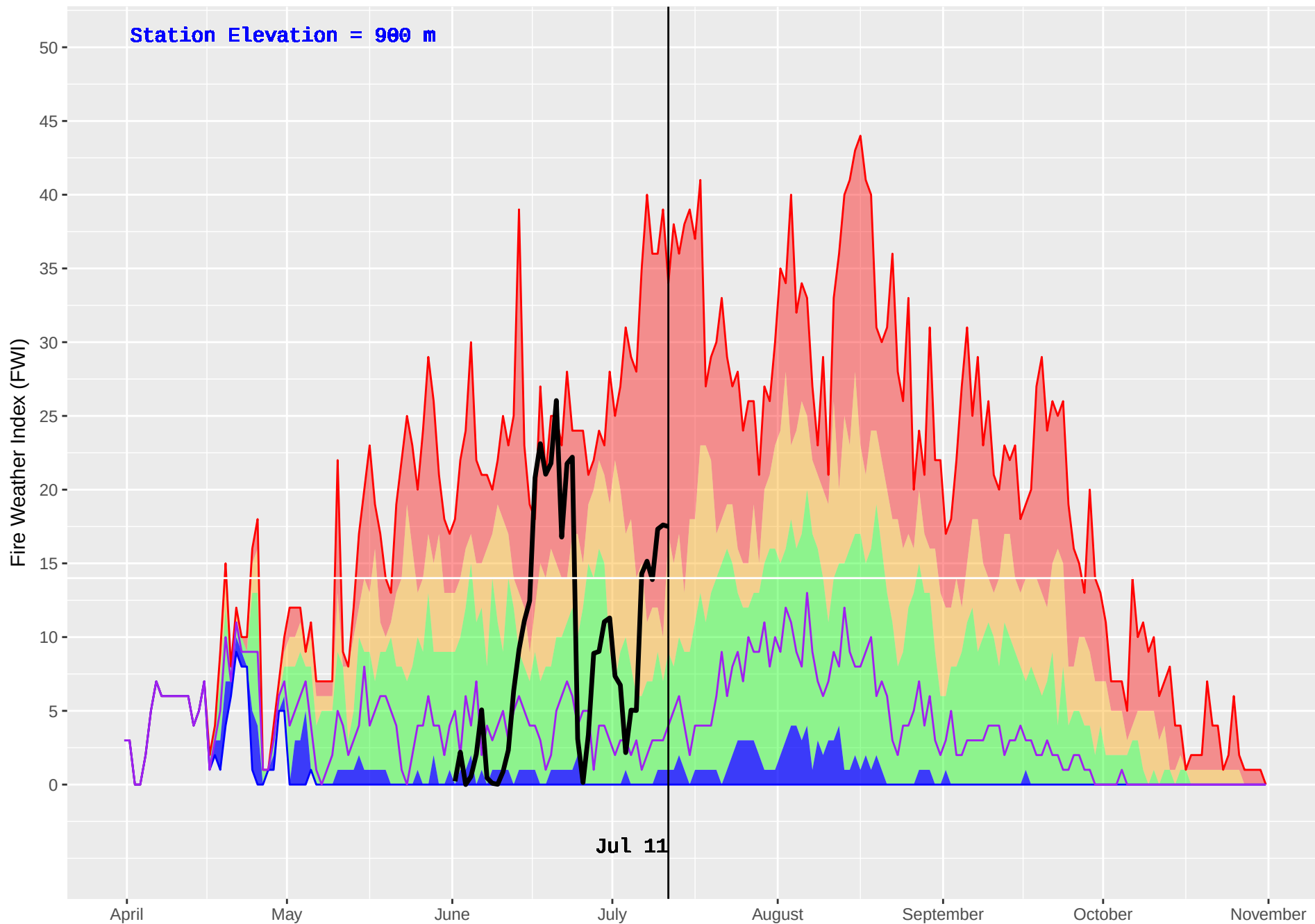
UPPER FULTON (169) : Historical (1986–2016) and Current (2018) Noon Fire Weather Index (FWI)
